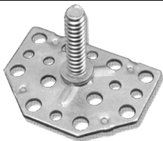
As Shown: M1-HP44-1/4-20x1.000
