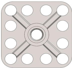
As Shown: F2-SB50-3/8-16x0.500
