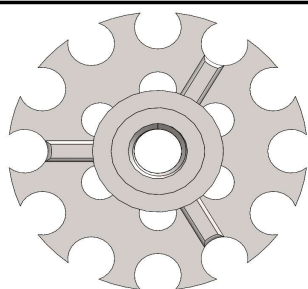
As Shown: F2-RB32-1/4-20x0.625
